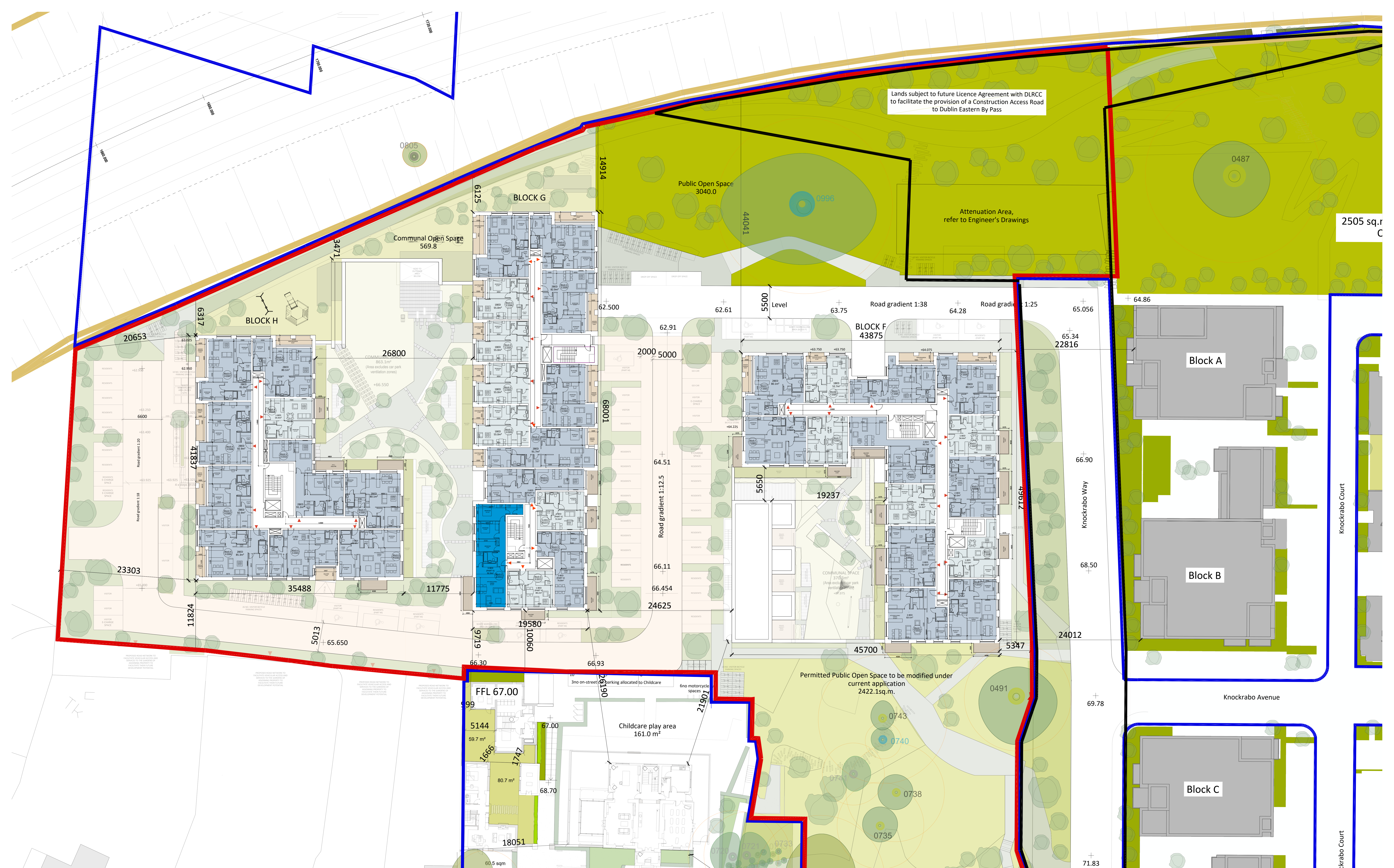
Block F, G & H Floor Plans, Level 03 PLEASE REFER TO ENGINEER'S DRAWINGS FOR PROPOSED ROAD LEVELS & SITE SERVICES LAYOUT AND TO LANDSCAPE ARCHITECTS DRAWINGS FOR LANDSCAPING PROPOSALS & PROPOSED BOUNDARY TREATMENTS. ALL DIMENSIONS IN MILLIMETERS
